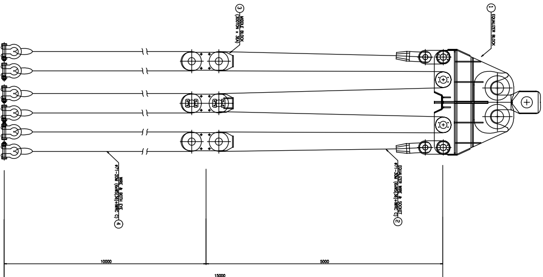
300 TON SLING ARRANGEMENT 6 POINT LIFTING / 1 HOOK
