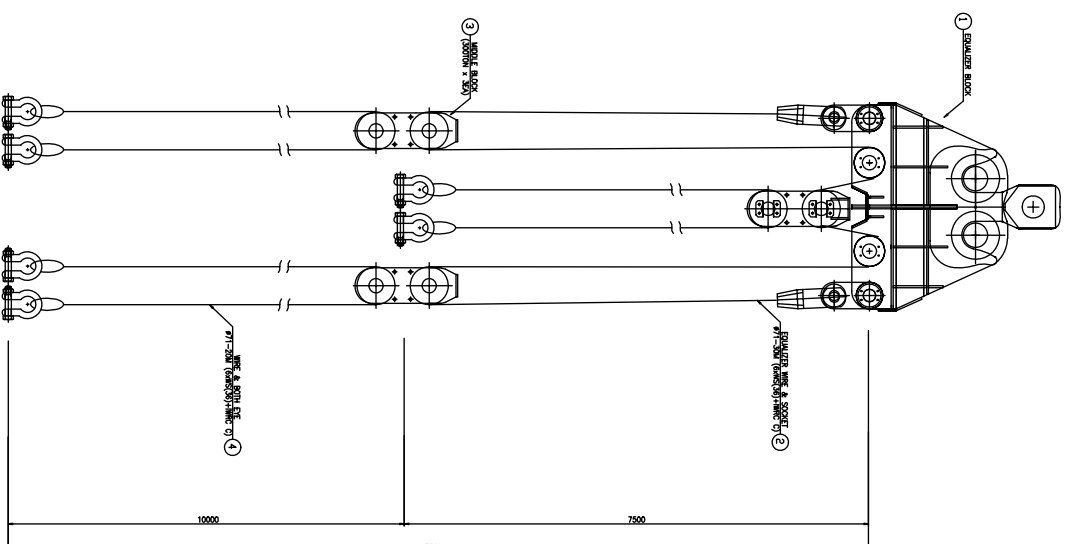
300 TON SLING ARRANGEMENT 4 POINT LIFTING / 1 HOOK
