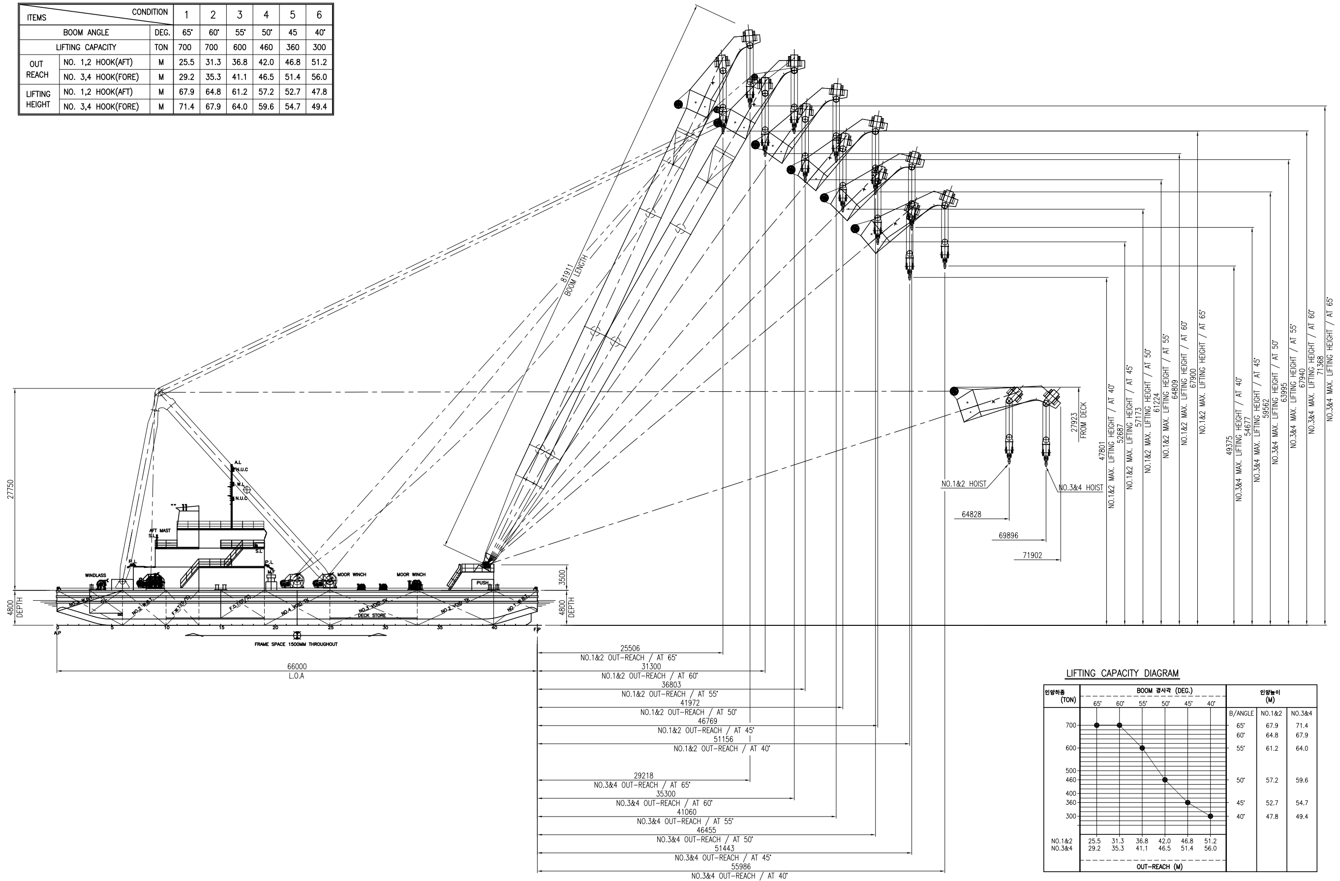
LIFTING CAPACITY TABLE
